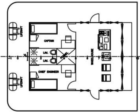
WHEELHOUSE DECK
